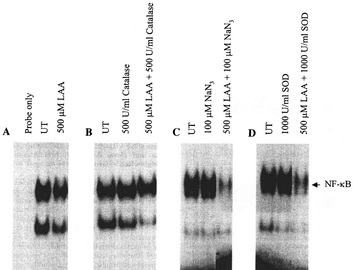
Fig. 6. LAA inhibits the activation of NF- \kappa B through H_2O_2 generation but not superoxide anion. HL-60 cells ( 7 \times 10^6 ) were cultured with or without 500 \mu M LAA, in the presence or absence of 500 U catalase per ml, 100 \mu M NaN_3 , or 1,000 U SOD per ml, as indicated for 24 h. Cells were harvested and nuclear extracts were extracted. Nuclear extracts (10 \mu g) were incubated with radiolabeled NF- \kappa B oligonucleotide at room temperature for 20 min and EMSA was performed as described in Materials and
